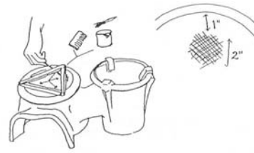
80. Place the triangle template so that one point is on the side of the firebox. Mark inside underneath the points. One inch below the rim, score and slip a 2" diameter area.
